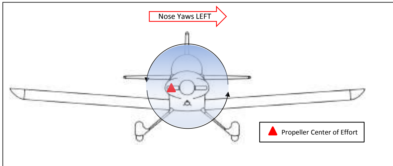
Figure 3-13: Engine Effect—P-Factor
