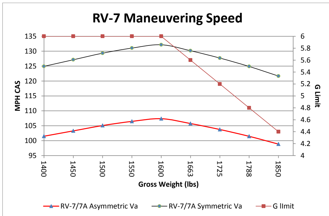
Figure 3-8: RV-7 Maneuvering Speed and G-Allowable (G Limit) vs Gross Weight. Derived from Van's Aircraft published performance data for RV-7/7A. All two-seat RV-types exhibit similar relationships.
