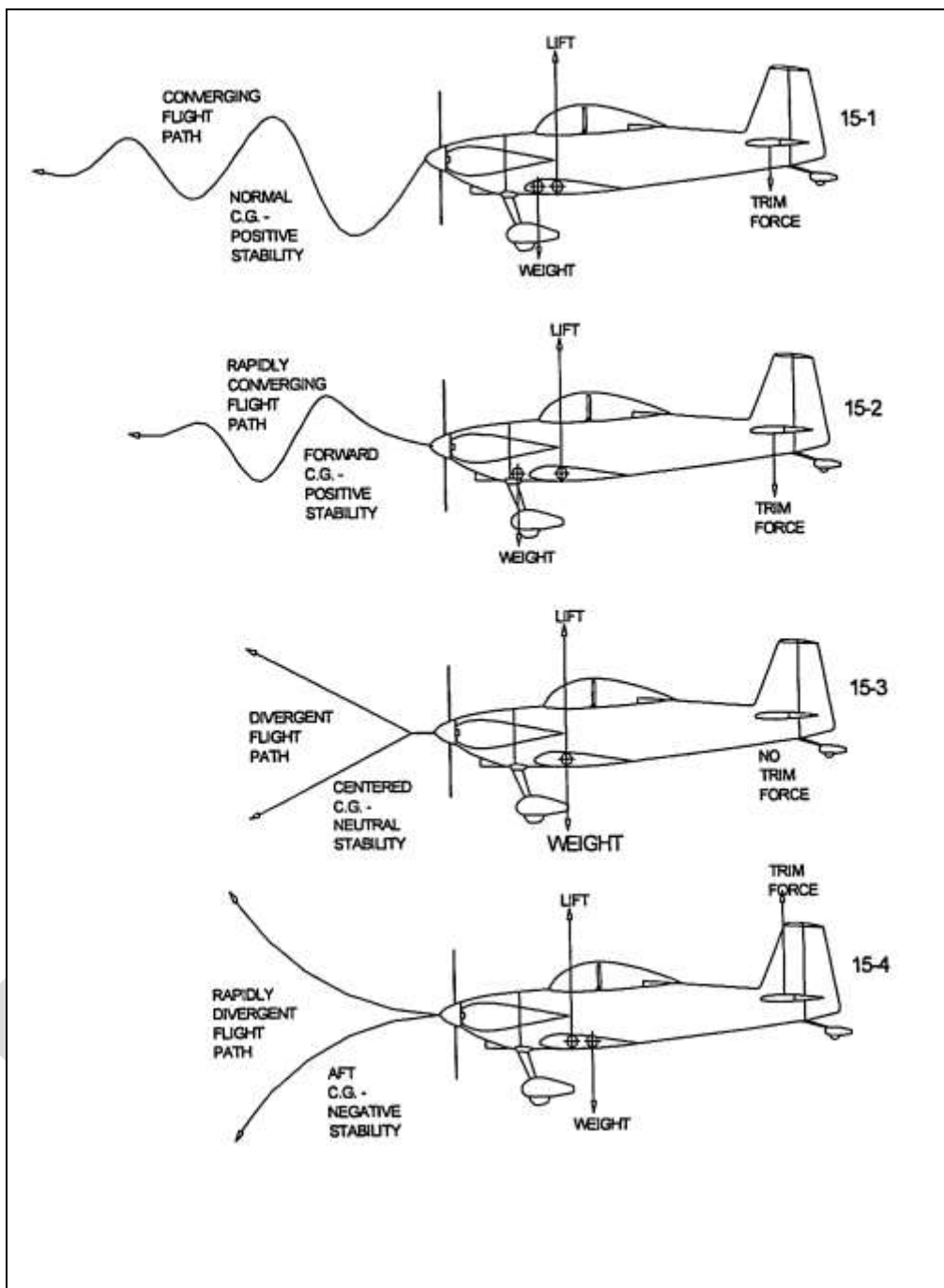
Figure 3-6. Basic aircraft stability.
