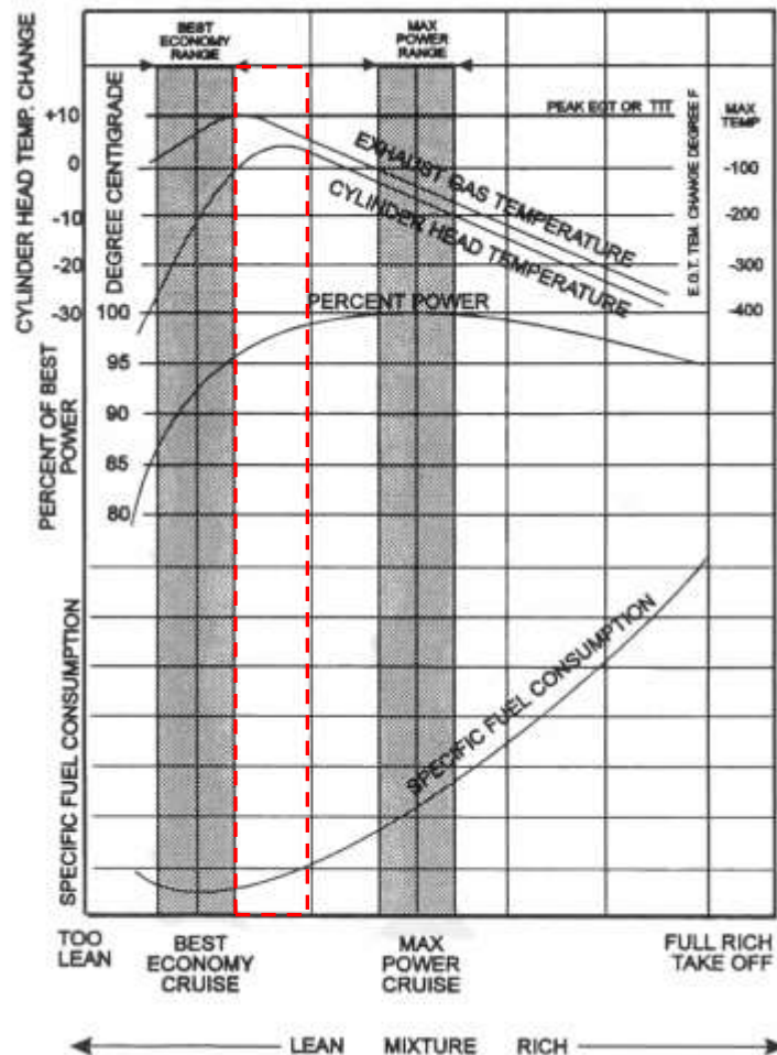
Figure 3-1. Typical Lycoming Installation: Effect of leaning on CHT, EGT, power and specific fuel consumption at constant engine RPM and manifold pressure. The red dashed area is peak EGT to 50° rich-of-peak (ROP). Operation in this area should be avoided.
