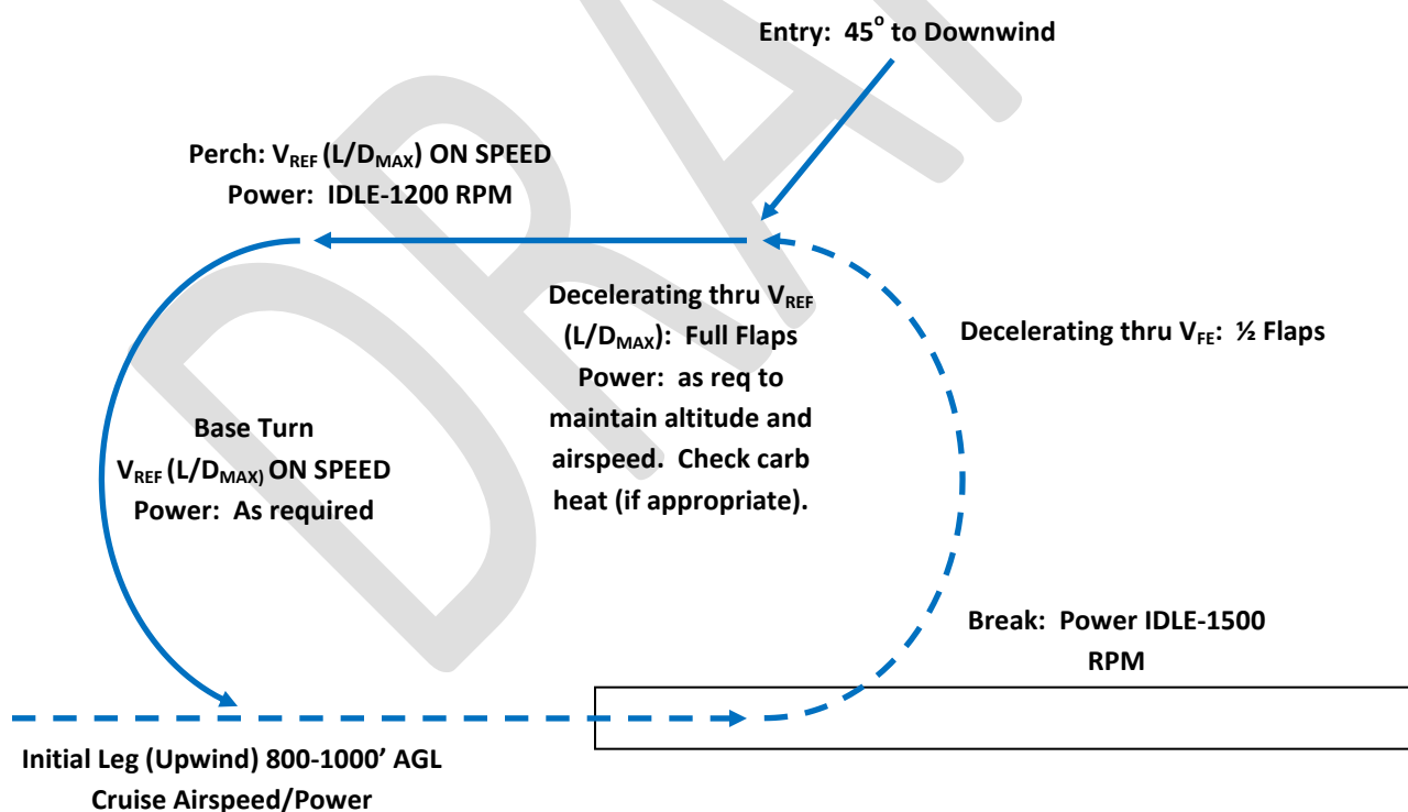
Figure 3-2. Normal Landing Pattern
