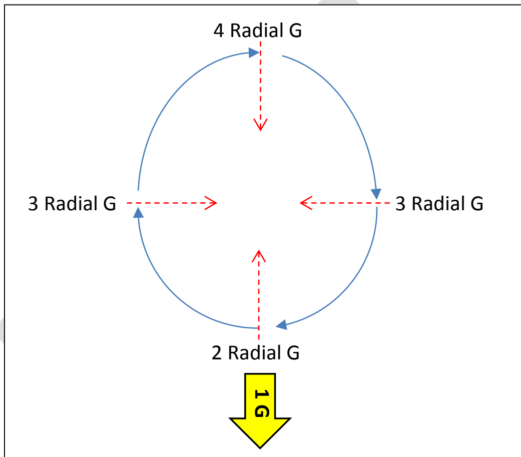
Figure 3-11. Constant 3 G Vertical Turn
