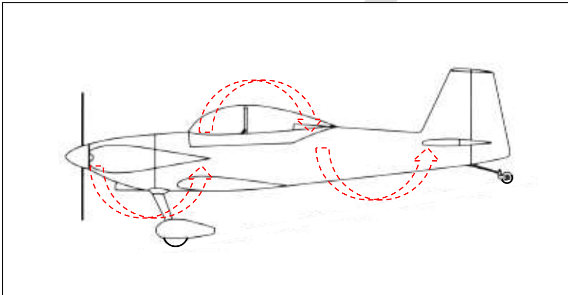
Figure 3-12: Propeller Effect—Spiraling Slipstream
