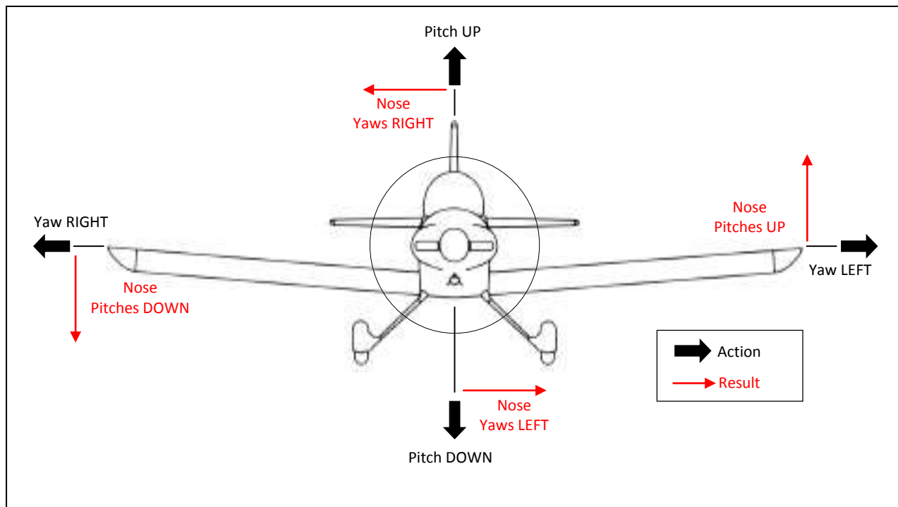
Figure 3-14: Propeller Effect—Gyroscopic Precession
