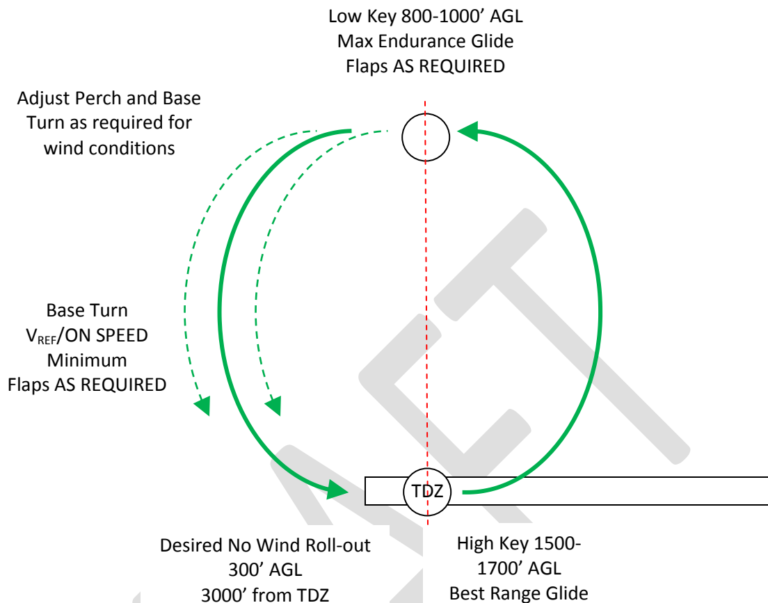
Figure 3-5. Emergency Landing Pattern.
