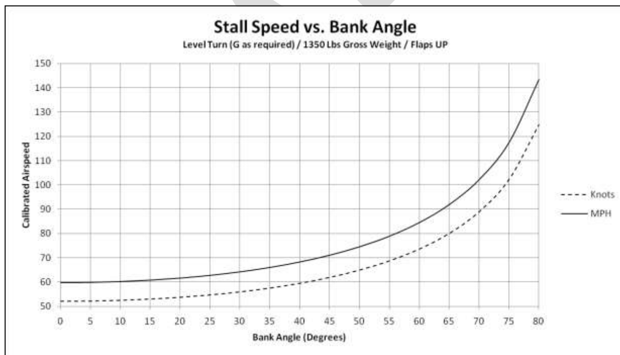
Figure 3-7. Example of Bank Effect on Indicated Stall Speed (1G calibrated stall speed is 60 MPH/53 Knots in this example).
