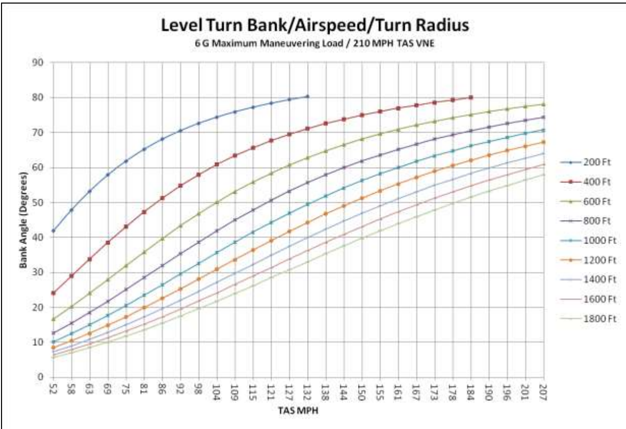
Figure 3-9. Bank and Airspeed Effect on Turn Radius (Level Turn)
