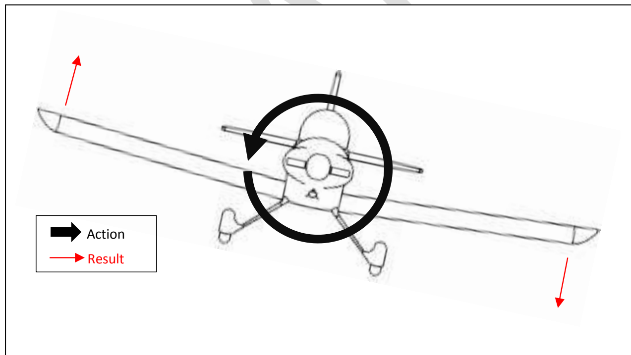
Figure 3-15: Propeller Effect—Torque
