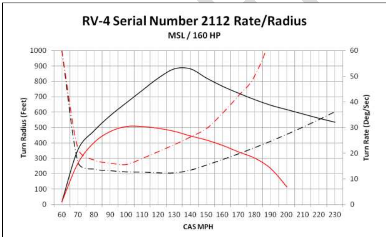
Figure 3-10. Example Turn Rate/Radius Diagram for an RV-4. Instantaneous turn performance is black and sustained turn performance is red. Turn rate (deg/sec) are the hill shaped curves and turn radius (feet) are the valley shaped curves. Maximum rate and minimum radius = best turn performance.
